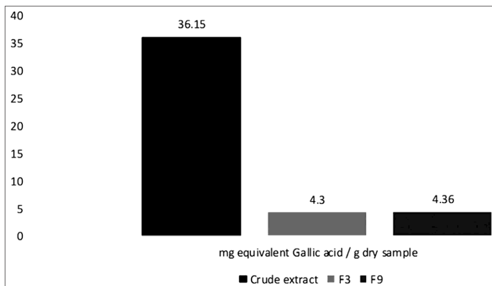
Figure 1: Level of total phenolic content crude extract, F3, and F9
