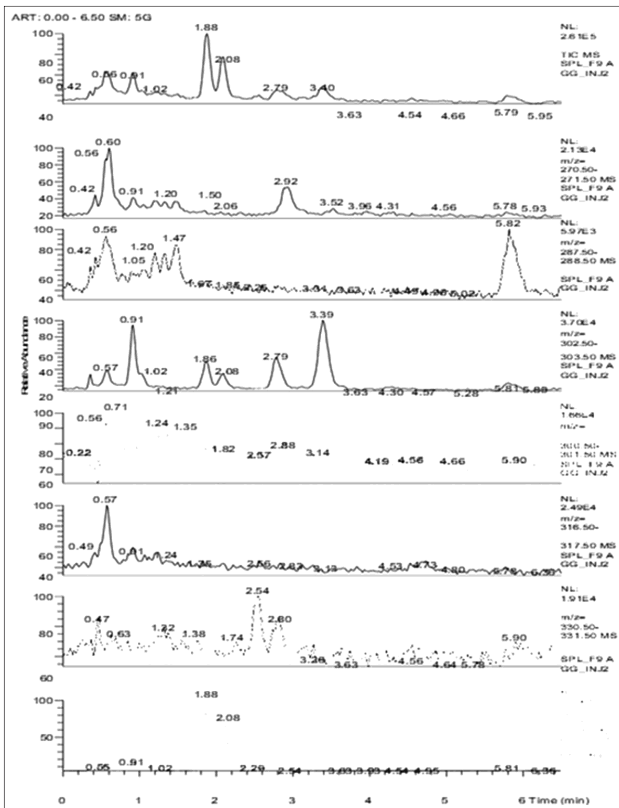
Figure 4: Liquid chromatography-mass spectrometry reading to identify a molecule from crude extract, F3, and F9
