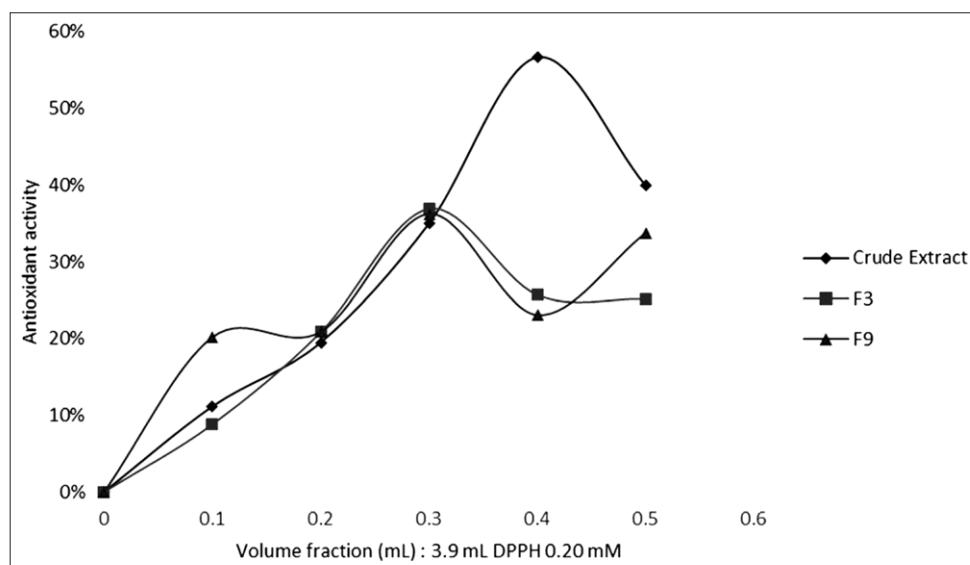
Figure 3: Antioxidant activity from crude extract, F3, and F9
